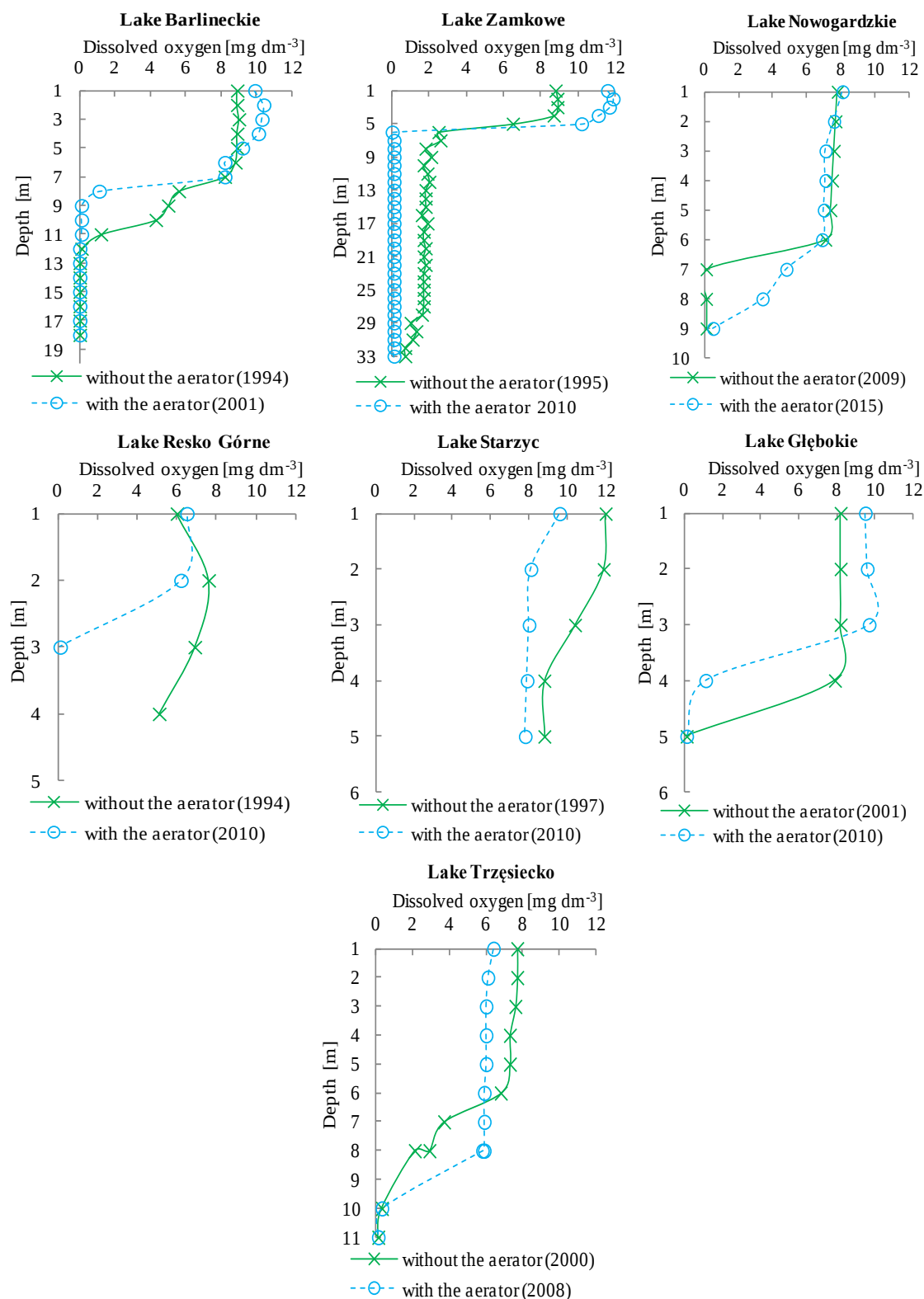
Figure 1. Example vertical profile of dissolved oxygen concentration in the water column at the deepest site of the lakes, in the summer season, before and after installation of the aerator.
